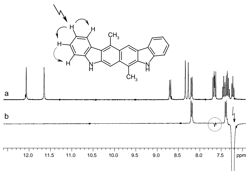
Figure 1. upper trace: downfield region of the 300 MHz ^1\text{H} -NMR spectrum of 7 (DMSO- d_6 , 28°C); lower trace: NOE difference spectrum of 7 ; irradiation of H-11: positive effects for H-10 and H-12, negative effect for H-9 (“three-spin effect” [cf. lit., 19 ]).
