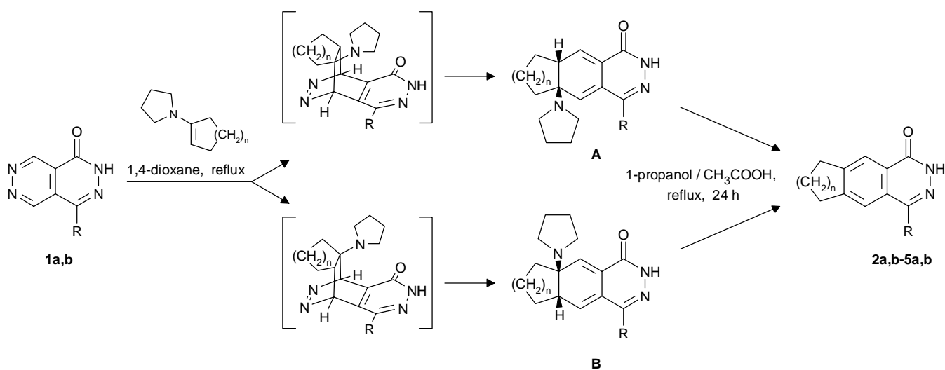
Scheme 1
